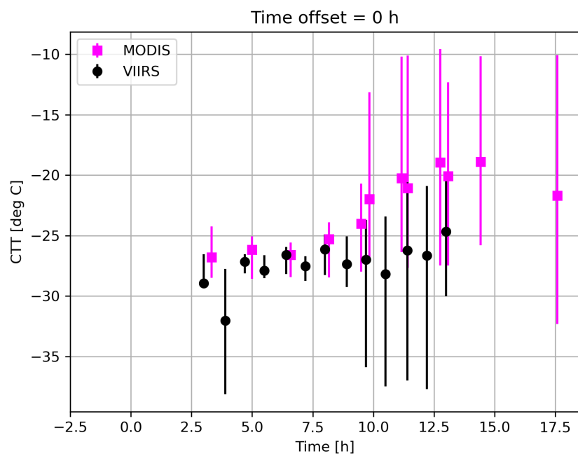
Figure C2. MODIS and VIIRS collocated brightness temperatures to infer cloud-top temperature show signs of surface contamination, evidenced by the large uncertainty bars. Mean values and bars are greater for MODIS that has a larger pixel size compared to VIIRS.
