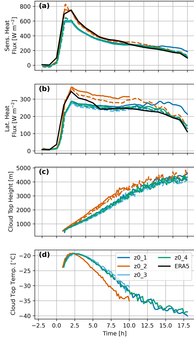
Figure C1. LES output using various surface roughness length configurations for DHARMA (solid lines) and WRF (dashed lines).
