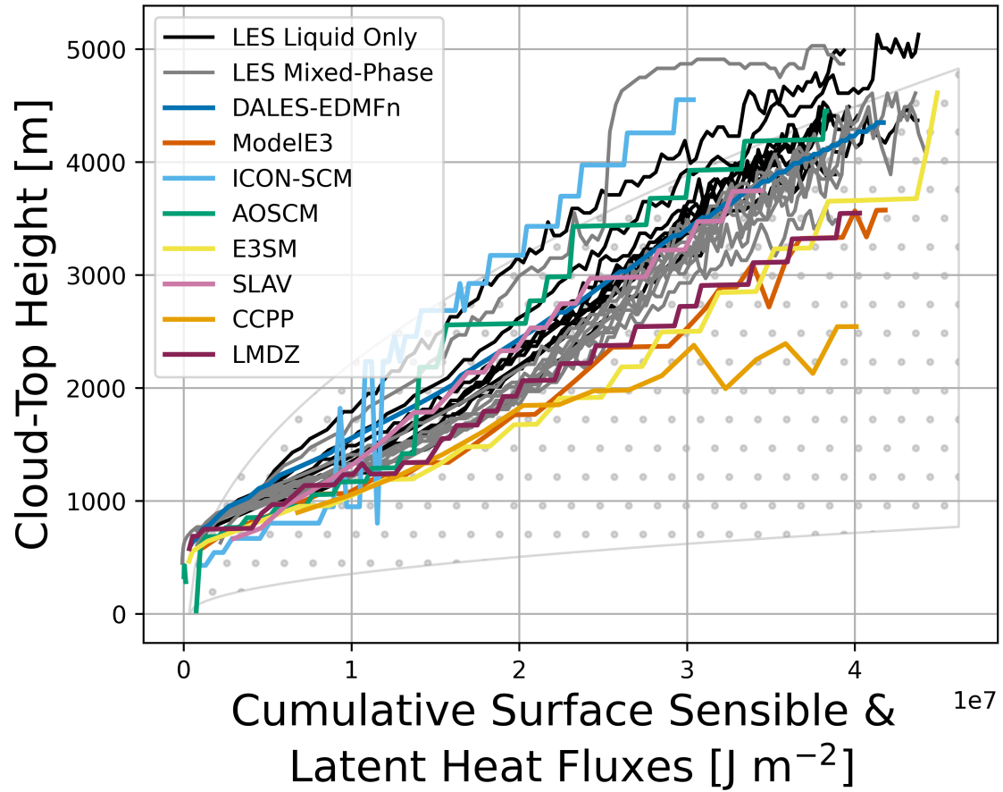
Figure 9. Relationship between cumulative surface heat (sensible and latent) fluxes and cloud-top height. LES Liquid Only and LES Mixed-Phase simulations are shown in the black and gray lines respectively, with each line representing results from a single model, while the SCMs are colored according to the legend. Stippling in the background shows theoretical expectations assuming surface-only forcing (Equ. 11.2.2f in Stull, 1988) under weakest and strongest conditions.
