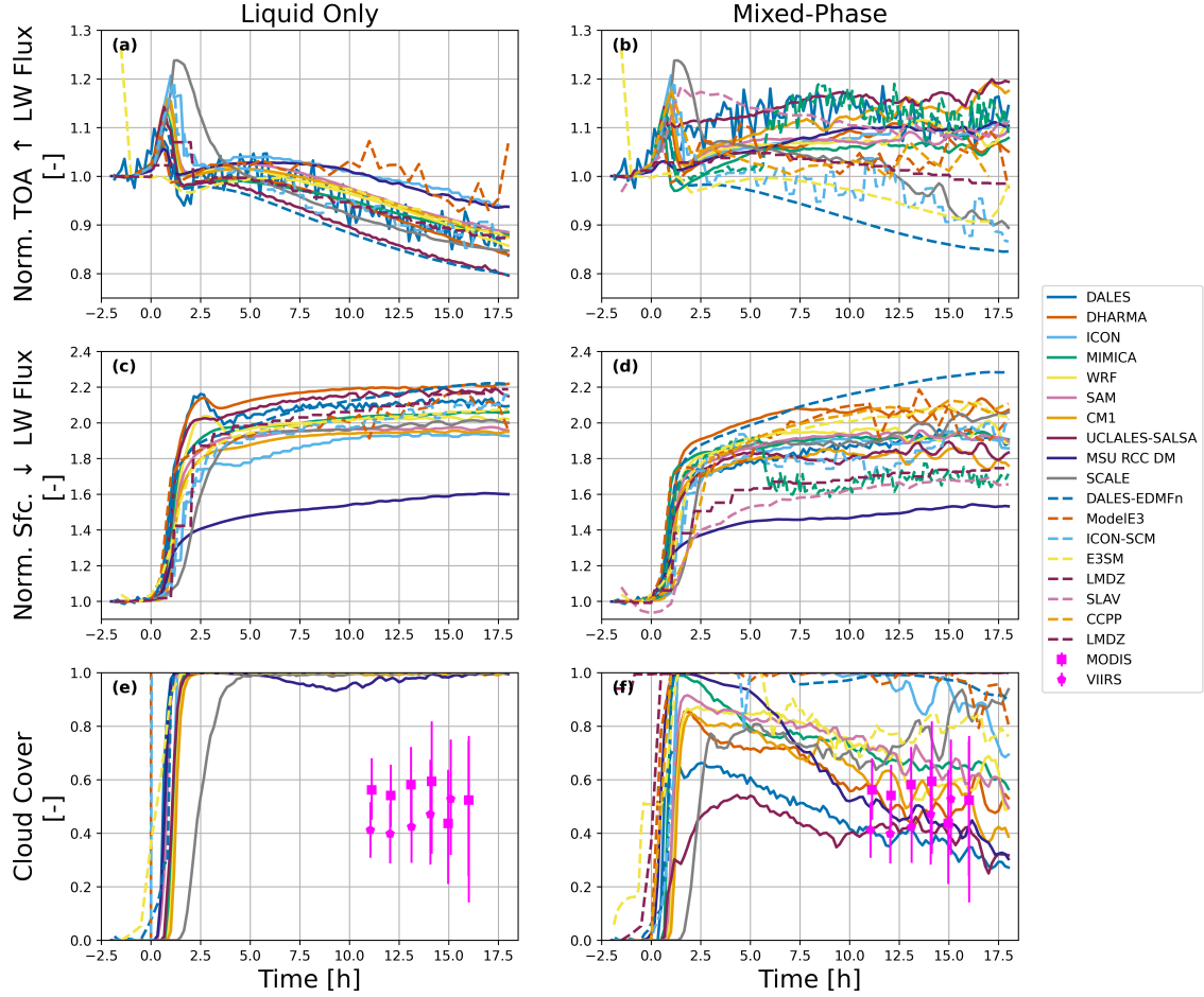
Figure 11. As in Fig. 10, except showing only model results that are normalized by the pre-cloud ( t=-1 h) values. In the bottom-most row, we also show the modeled cloud cover together with observational targets, inferred from satellites carrying the MODIS and VIIRS instruments. Identical to LES, cloud cover is computed as the portion of pixels with a cloud optical depth greater than 2.0.
