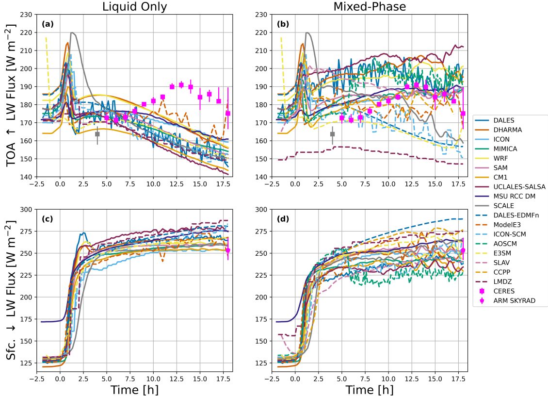
Figure 10. Time series of (top row) TOA upwelling LW fluxes and (bottom row) surface downwelling LW fluxes for (left column) Liquid Only simulations and (right column) Mixed-Phase simulations. LES models (solid lines) and SCMs (dashed lines) are colored according to the legend. ARM SKYRAD and CERES observations co-located with the model domains in space and within 1 h time are shown by the magenta markers. The gray marker represents a CERES retrieval potentially biased by a high solar zenith angle. The markers represent the mean value spanning the LES domain while the bars represent the interquartile range.
