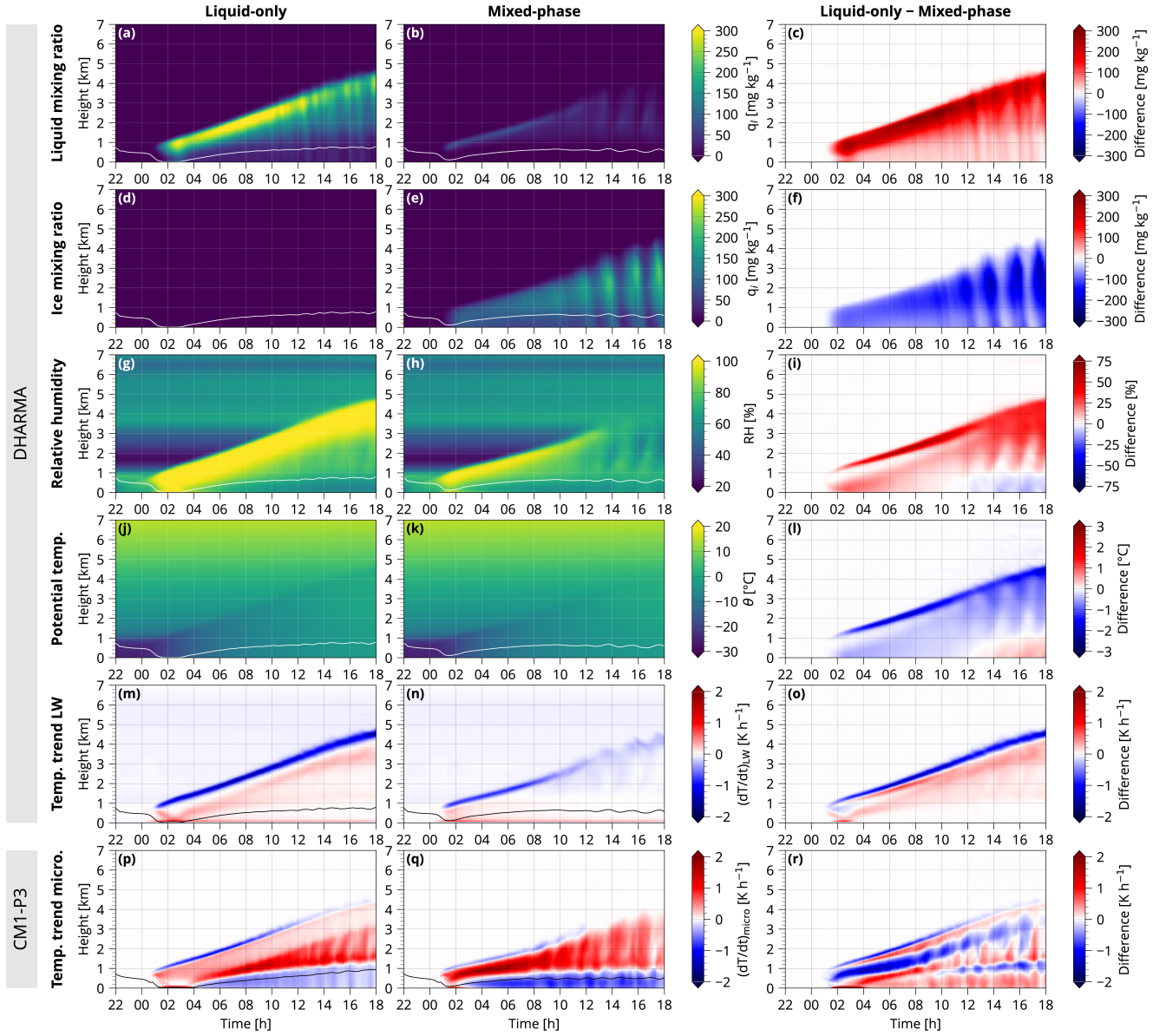
Figure D1. Curtain plots of liquid and ice mixing ratios (cloud plus precipitation), relative humidity (relative to liquid), potential temperature, temperature trend due to longwave radiation, and temperature trend due to microphysics in the DHARMA and CM1-P3 simulations for the liquid-only case, mixed-phase case, and their difference. The white and black lines show the lifting condensation level.
