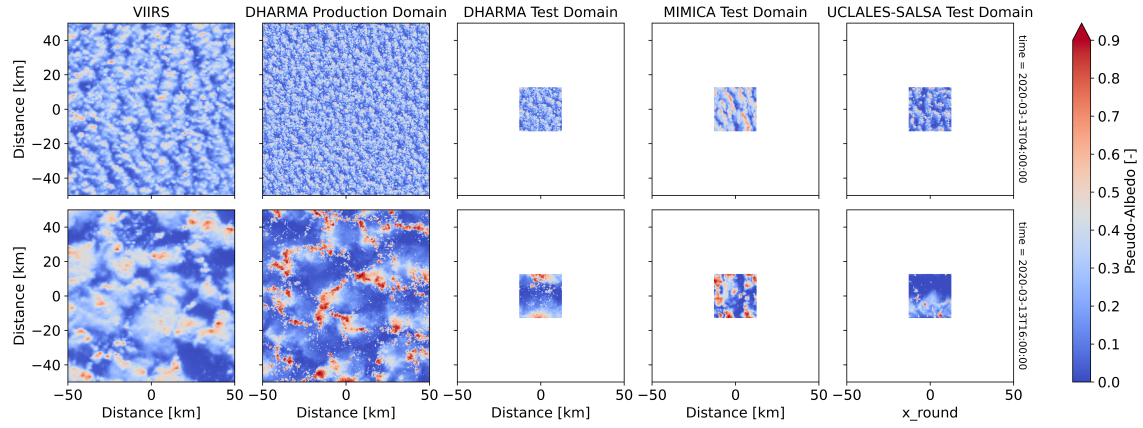
Figure 7. Pseudo-albedo comparison between VIIRS and DHARMA, MIMICA, and UCLALES-SALSA LES models at (top) 0400 UTC (rolls) and (bottom) 1600 UTC (cells).
