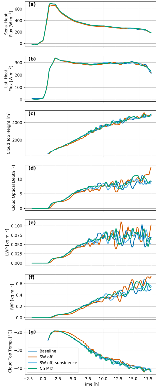
Figure B1. DHARMA LES output using various physics options.
