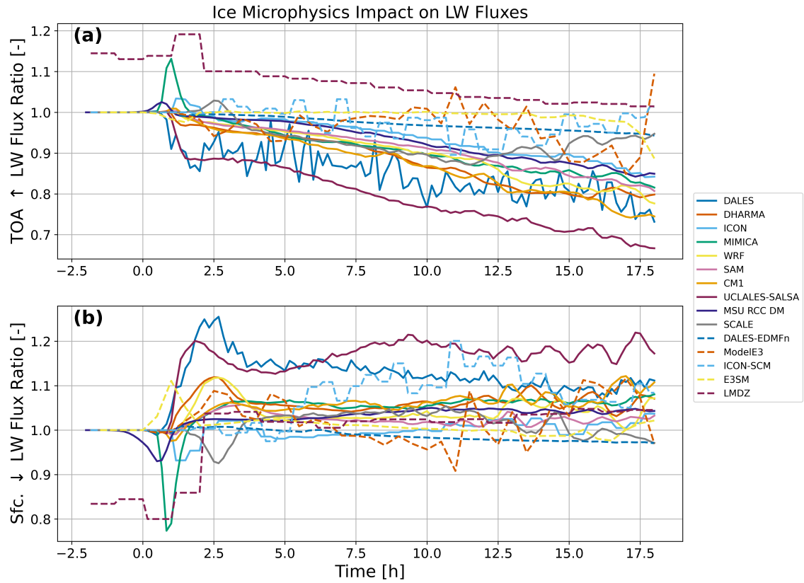
Figure 12. Time series of (top row) TOA upwelling LW flux ratio and (bottom row) surface downwelling LW flux ratio. The ratio is computed as the Liquid Only result divided by the Mixed-Phase result. That is, for a given model, a ratio value larger than 1 indicates that the value of the respective variable is larger in the Liquid Only simulation than in the Mixed-Phase simulation.
