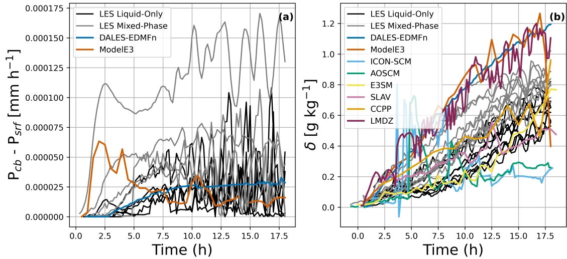
Figure 6. Cloud-base minus surface precipitation rate (left) and water vapor mixing ratio difference between the bottom and top of the MBL (i.e., 25% and 75% of cloud-top height, respectively) (right) over time. LES Liquid Only and LES Mixed-Phase simulations are shown in the black and gray lines respectively, with each line representing results from a single model, while the mixed-phase SCMs are colored according to the legend, noting that not all models reported precipitation flux profiles.
