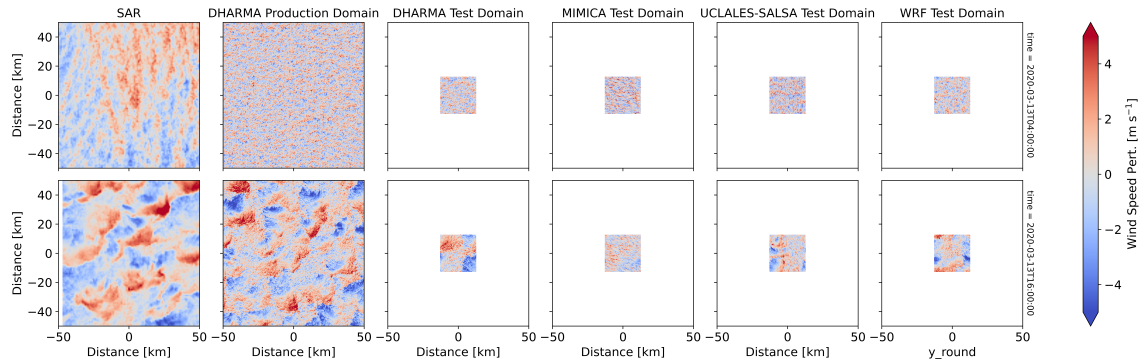
Figure 8. 10 m wind speed perturbation comparison between SAR and DHARMA, MIMICA, UCLALES-SALSA, and WRF LES models at (top) 0400 UTC (rolls) and (bottom) 1600 UTC (cells). The 10 m wind speed perturbation field is computed by subtracting the domain-averaged value from each grid cell.
