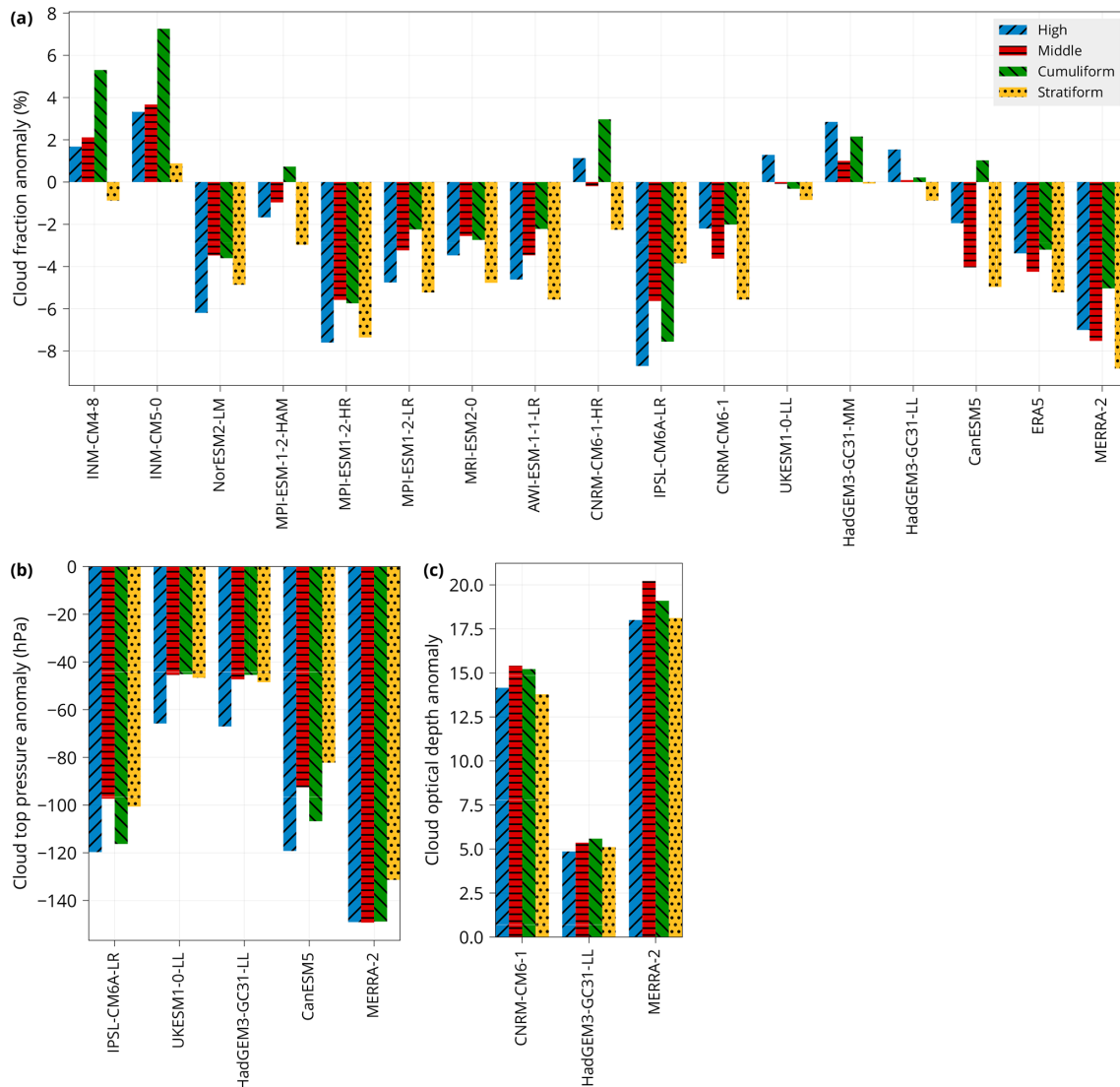
Figure 9. Cloud properties in CMIP models and reanalyses by cloud type relative to CERES. The bar charts show area-weighted global means of cloud properties calculated over the domain where cloud types are determined by the ANN (all locations except polar regions in winter). Cloud properties shown are (a) cloud fraction, (b) cloud top pressure and (c) cloud optical depth. In the CMIP models, cloud top pressure is from the ISCCP simulator. All other cloud properties are from non-simulator variables. For each cloud type, the mean is calculated from daily data by weighting values by the cloud type occurrence determined by the ANN for the particular model or CERES in every grid cell and time step. The model and reanalysis data are for the years 2003–2014, and the CERES data are for the years 2003–2020. The models are sorted by their ECS from lowest to highest.
