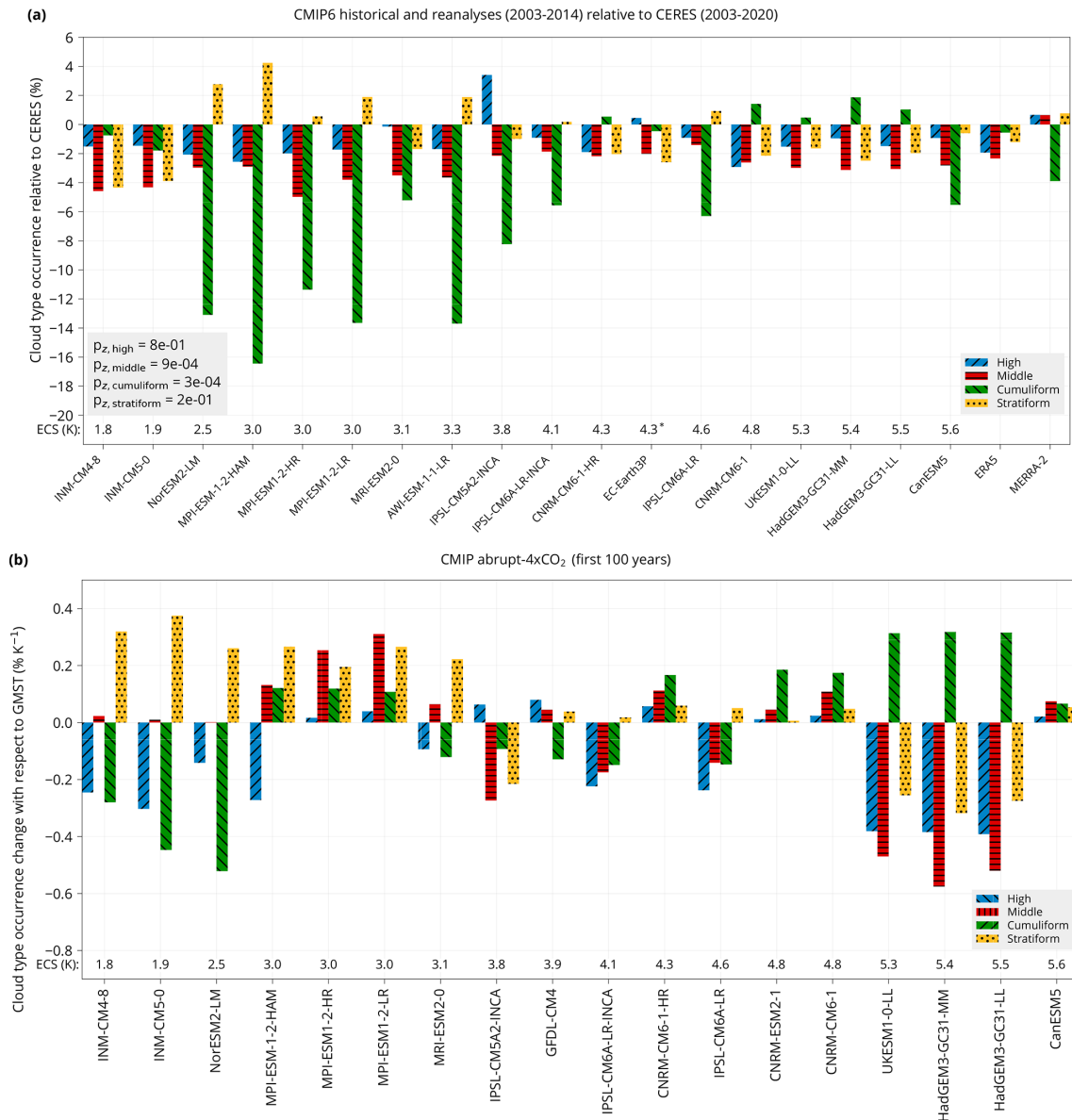
Figure 8. (a) Global mean cloud type occurrence in CMIP6 models and reanalyses relative to CERES in the historical experiment. Shown is also the p value of a z test for the difference in the means of two groups of CMIP models with ECS below and above 4 K (the mid-point ECS in the range of the analysed models). (b) Global mean of cloud type occurrence change with respect to global mean near-surface air temperature (GMST) in CMIP5 and CMIP6, calculated by linear regression. Models are sorted by their equilibrium climate sensitivity (ECS). For some models, marked by “*”, ECS was not available and was taken from a related available model (see Table 1).
