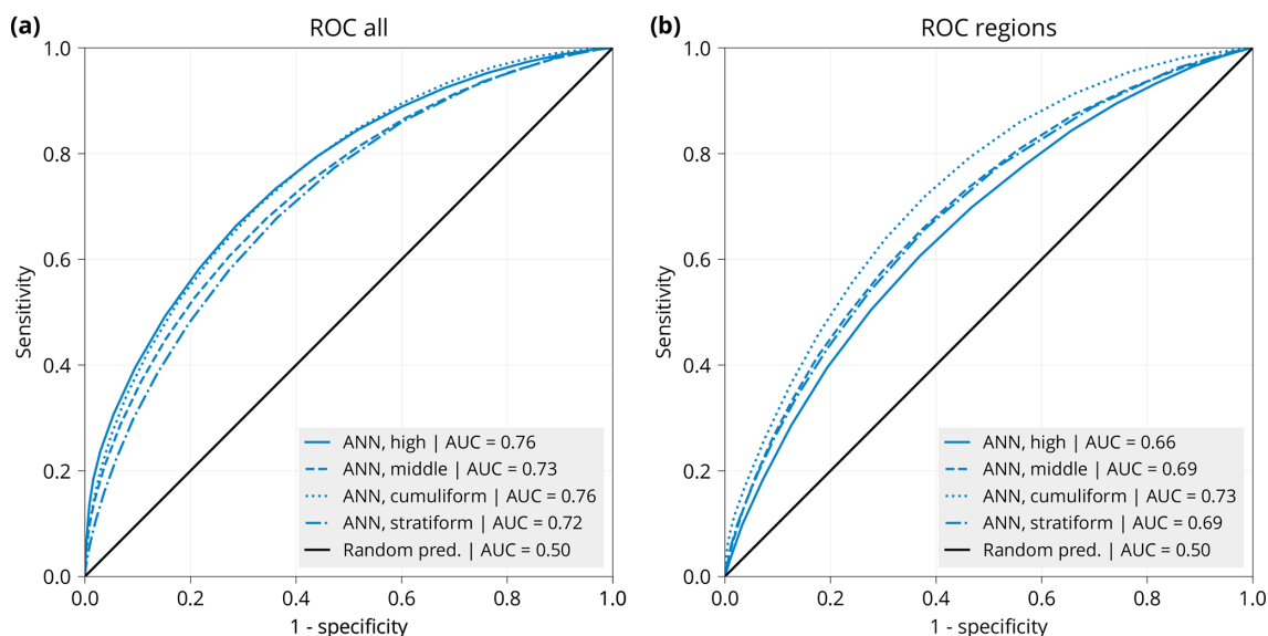
Figure 5. Receiver operating characteristic (ROC) diagram calculated for (a) an ANN for the four cloud types trained on all training years (2003–2020, except the validation years 2007, 2012 and 2017) on all data available globally, evaluated against station reports from the IDD in the validation years and (b) a composite of four ANNs trained on all training years on all data available globally except for each of the four validation regions (North Atlantic, East Asia, Oceania and South America), evaluated against station reports from the IDD in the respective region in the validation years. Shown is also the ROC of a random predictor. Sensitivity is the true positive rate (probability of a positive prediction if positive in reality), also called the hit rate. Specificity is the true negative rate (probability of a negative prediction if negative in reality). “1-specificity” is also called the false alarm rate. The area under the curve (AUC) of the ROCs is in the label.
