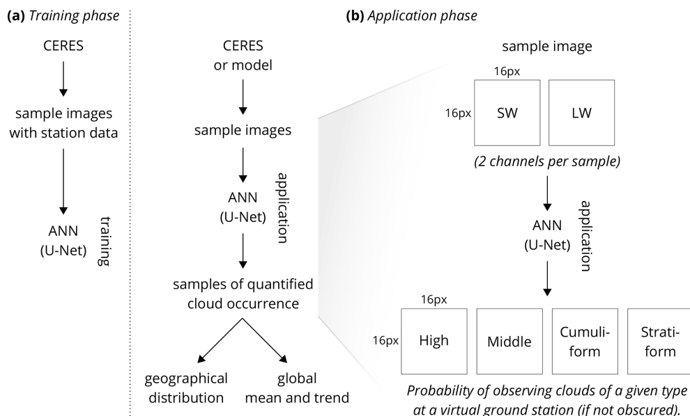
Figure 2. Schematic showing the principle of training and applying the ANN. (a) Sample images from CERES with reference ground station data (WMO cloud genera) are used in the training phase. (b) In the application (“prediction”) phase, the ANN quantifies cloud type occurrence in sample images from CERES or a model. The ANN takes a sample image consisting of SW and LW channels and produces per-pixel quantification of the probability of observing a given cloud type at a virtual ground station located in the pixel. The samples are 16 \times 16 pixels in size and 4000 \times 4000 km spatially.
