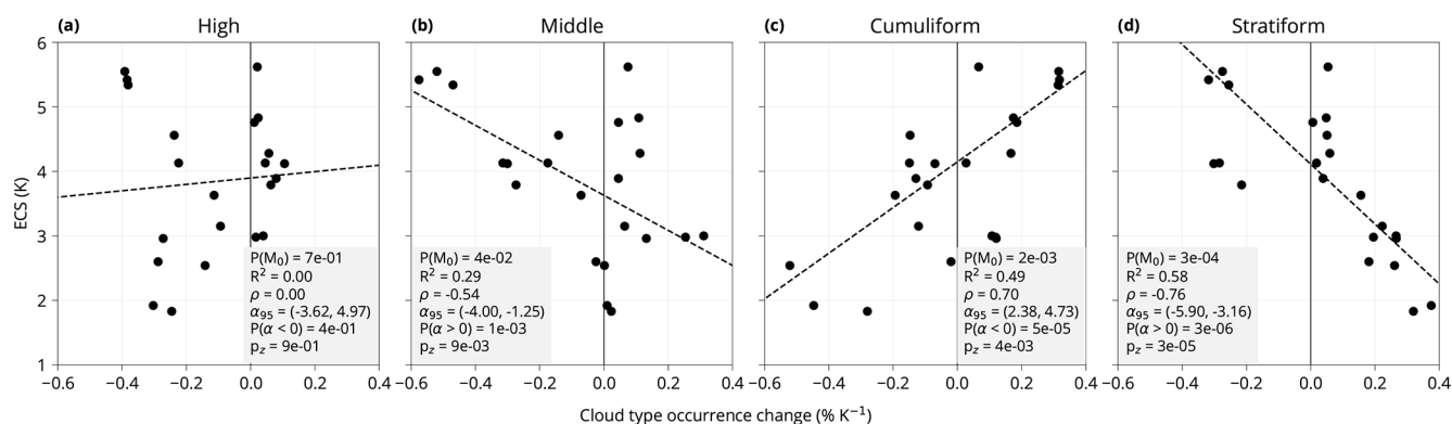
Figure 10. Dependence of model ECS on the cloud type occurrence change with respect to GMST. Confidence bands represent the 68 % range. Linear regression is calculated using Bayesian simulation assuming a Cauchy error distribution (Appendix A). Shown is also the probability of the null hypothesis model P(M_0) (explained in Sect. 4.6), the coefficient of determination ( R^2 ), the correlation coefficient ( \rho ), the 95 % confidence interval of the slope ( \alpha_{95} ) of the linear regression, the probability that the slope is smaller or greater than zero, P(\alpha < 0) and P(\alpha > 0) , and the p value of a z test ( p_z ) for the difference in the means of two groups of models in the bottom 50 % and top 50 % of ECS. For some models, marked with “*”, ECS was not available and was taken from a related available model (see Table 1).
