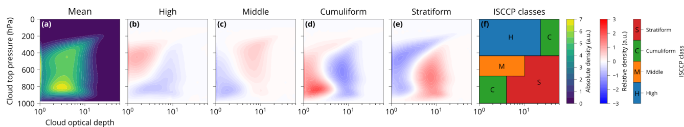
Figure 7. Histogram of cloud optical depth and cloud top pressure of the cloud types derived from CERES (2003–2020) by applying the ANN. (a) Mean of the four cloud types. (b–e) Difference from the mean for the classification of four cloud types. (f) ISCCP classification (Rossow and Schiffer, 1991).
