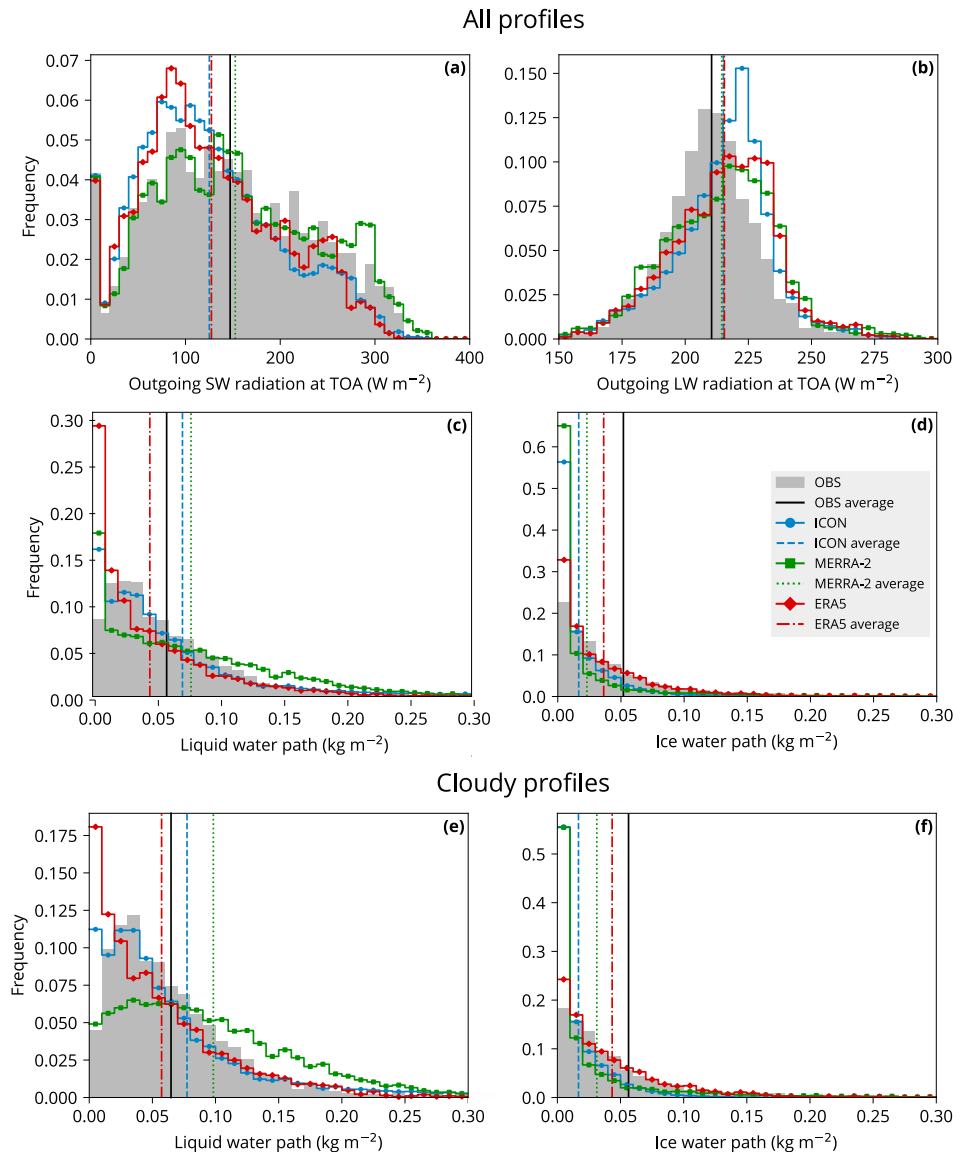
Figure 9. Histograms and averages of outgoing (a) SW, (b) LW radiation at TOA, (c), (e) liquid water path, and (d), (f) ice water path in CERES SYN1deg observations (OBS), ICON, MERRA-2, and ERA5. The results are shown for (a)–(d) all and (e), (f) cloudy profiles. All campaigns are weighted equally. The statistics are calculated from daily mean values corresponding to each time step and geographical location of the voyage tracks and stations.
