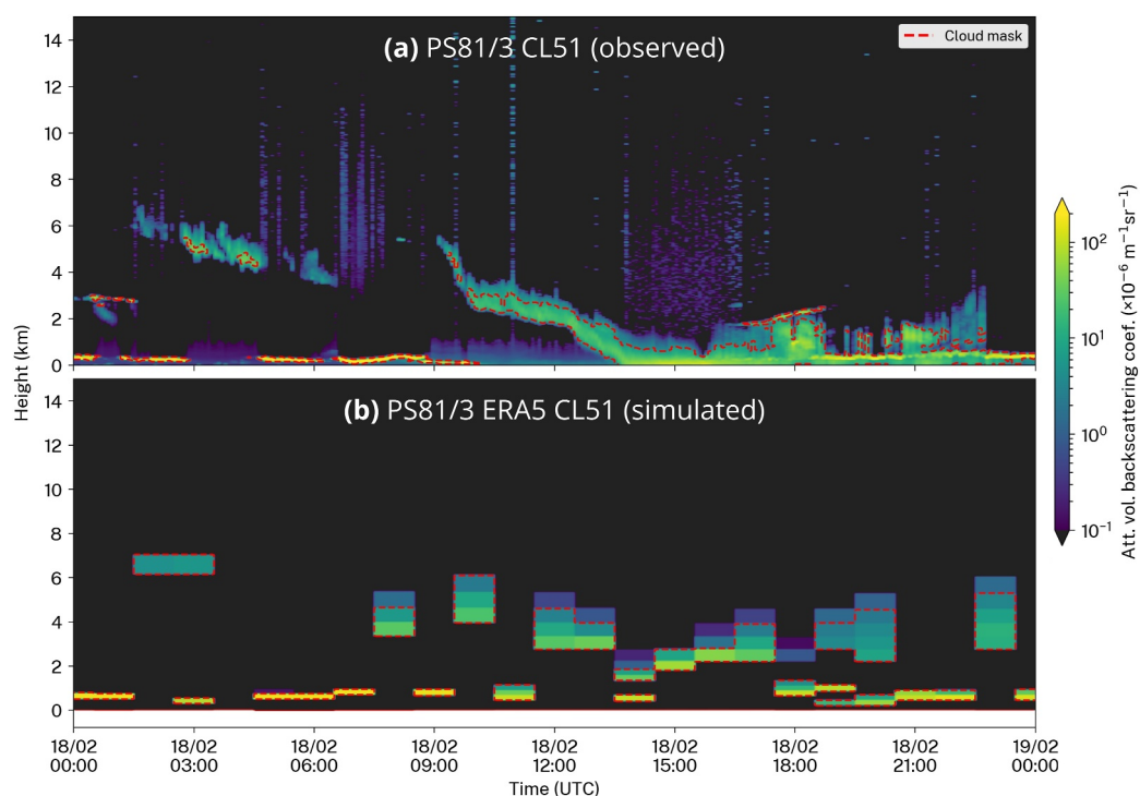
Figure 2. An example of the attenuated volume backscattering coefficient (AVBC; a) measured by the CL51 during 24 hr on the PS81/3 voyage and (b) an equivalent AVBC simulated with the ALCF from ERA5 data during the same time period. The red line identifies the cloud mask determined by the ALCF.
