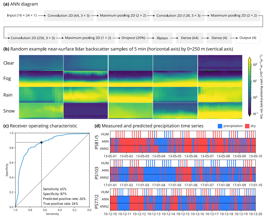
Figure 3. Artificial neural network (ANN) for prediction of precipitation in lidar backscatter. (a) Diagram showing the TensorFlow structure of the ANN, (b) randomly selected example samples of very low-level (0–250 m) backscatter in four categories (clear, fog, rain, and snow), as determined by coincident manual weather observations, (c) receiver operating characteristic diagram of the ANN, (d) examples of 10-day time series of human-observed (“HUM”) and predicted precipitation based on an ANN trained on all voyages (“ANN”) and all voyages except for the shown voyage (“ANN2”) during three randomly selected voyages with the available data. Here, by “randomly selected,” we mean selected from the top of a permutation generated by a pseudo-random number generator to prevent authors' bias in the selection.
