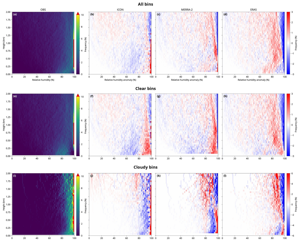
Figure 11. Relative humidity histograms calculated from the observed radiosonde profiles and the equivalent model and reanalysis profiles for (a–d) all bins, (e–h) clear bins, and (i–l) cloudy bins, determined from the lidar cloud mask. Model and reanalysis histogram values are relative to observations. The histogram values are normalized to 100% for each level separately. All campaigns are weighted equally.
