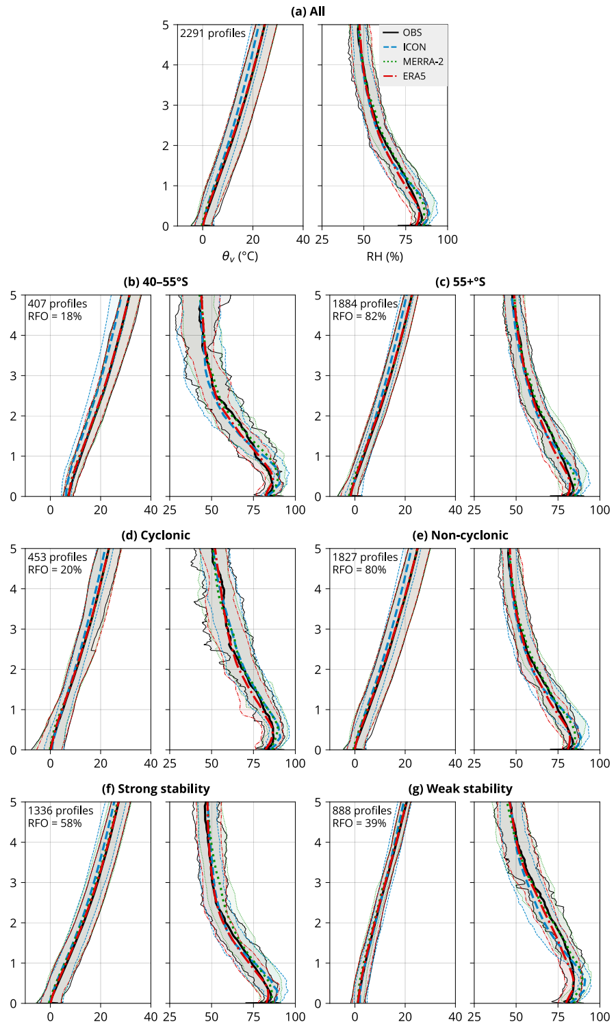
Figure 10. Virtual potential temperature ( \theta_v ) and relative humidity (RH) determined from radiosonde launches and co-located profiles in ICON, ERA5, and MERRA-2 in subsets as in Figure 7. The solid lines are the average calculated from the averages of every individual voyage and station. The bands span the 16th–84th percentiles, calculated from the distribution of the voyage and station averages. Shown is also the relative frequency of occurrence and the number of profiles in each subset.
