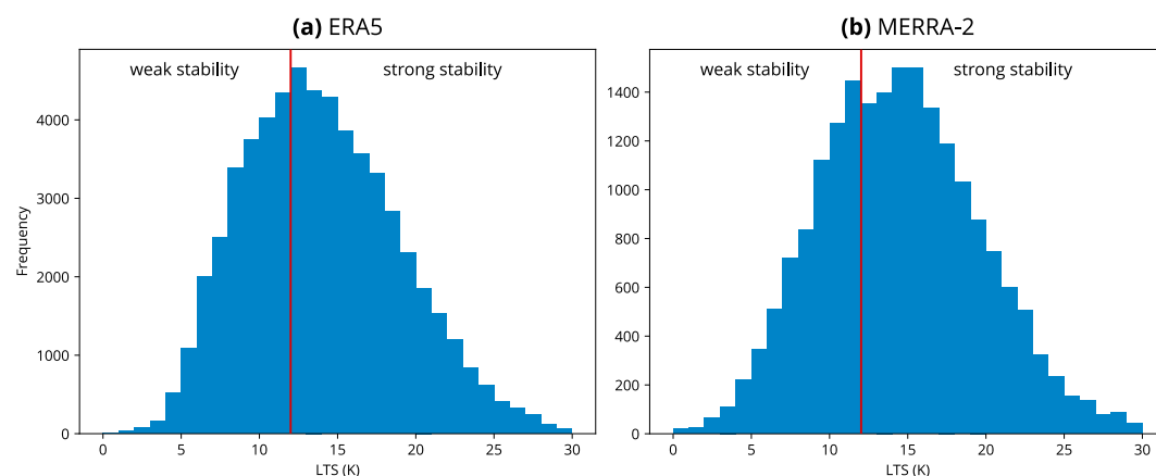
Figure 4. Lower tropospheric stability (LTS) distribution in panel (a) ERA5 and (b) MERRA-2 calculated for the 31 voyage tracks and one station from the highest instantaneous temporal resolution data available. Shown is also the chosen dividing threshold of 12 K for conditions of weak and strong stability.
